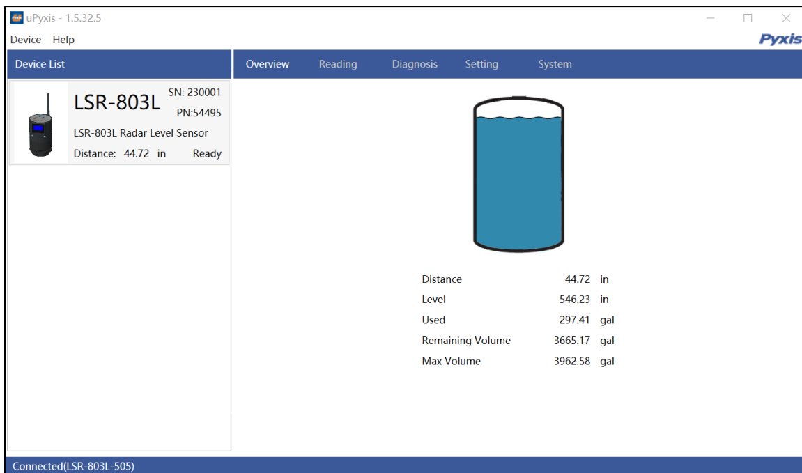
Figure 10. uPyxis Live Display After Connection to LSR-803L Series Sensor
