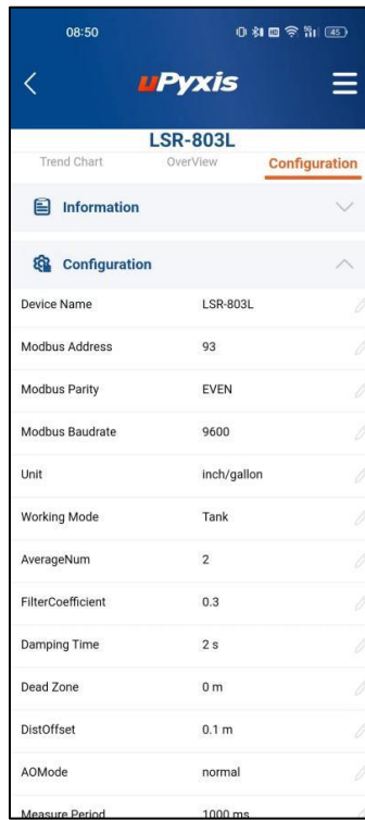
Figure 7. Sensor Configuration
