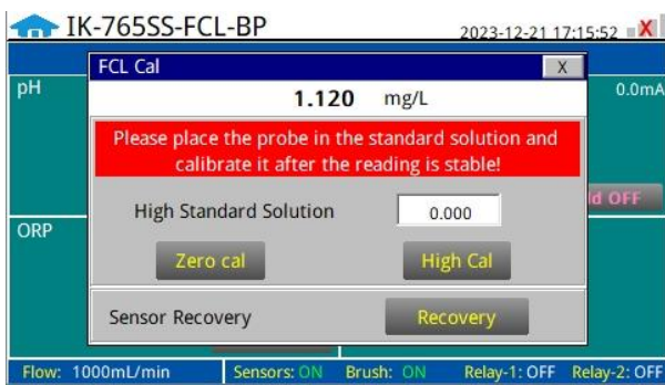
Figure. 46 – Free Chlorine Calibration of ST-765SS-FCL
