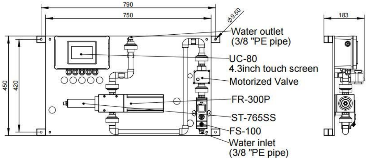
Figure. 1 - OxiPanel-PLUS IK-765SS-BP Series
