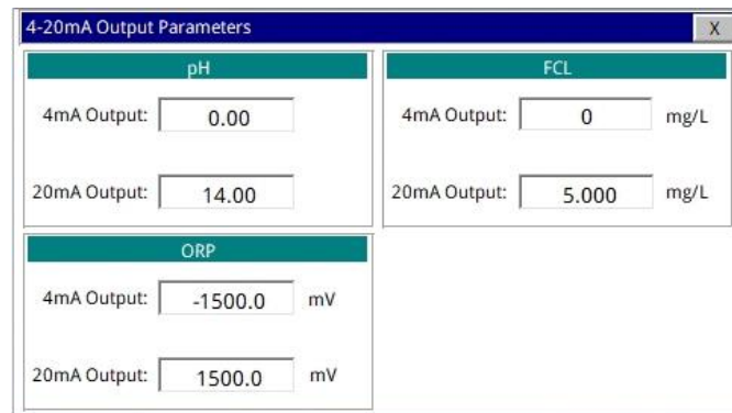
Figure. 39 - 4-20mA Output Setting
