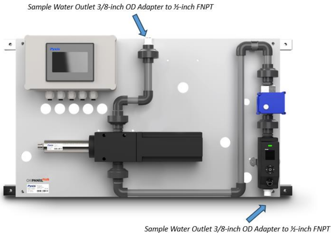
Figure. 2 Sample Water Inlet and Outlet Diagram
