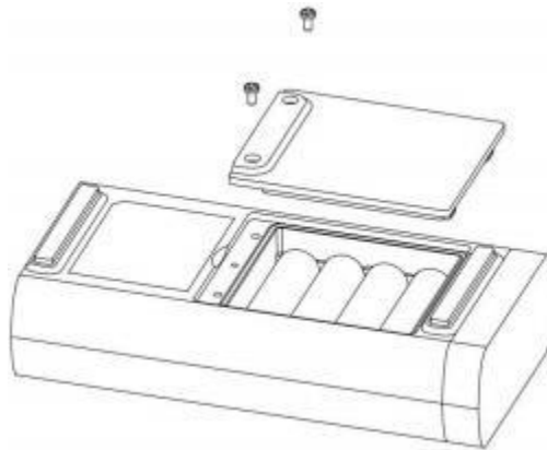
Figure 1. The SP-350RO battery compartment
