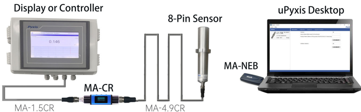
Figure 14. Bluetooth connection to LT-73X Series sensor with MA-CR, MA-NEB and uPyxis Desktop App.
