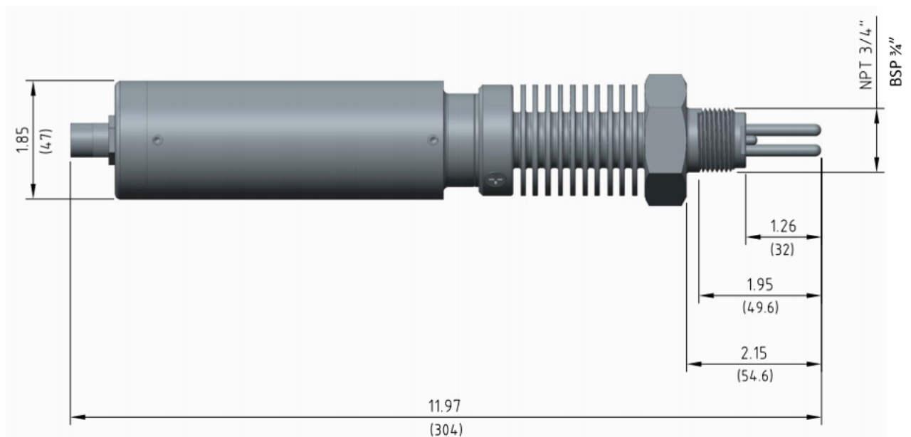
Figure 3. CR-301 Dimensions in Inch (mm)
